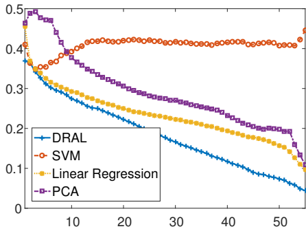
Figure 7: The MSE where \mathcal{D} is fully observed for Linear Regression, SVM, PCA and DRAL with Information Gain heuristic
