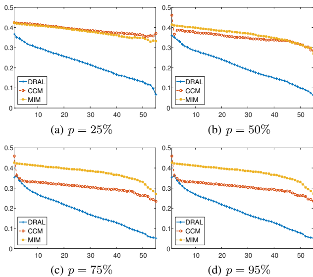
Figure 9: The MSE Linear Regression (CCM and MIM) and DRAL model (with Information Gain selection), where every entry of every record in \mathcal{D} is observed with probability p
