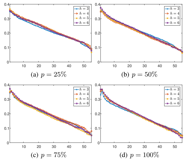
Figure 10: The MSE of different h values for the DRAL model with information, where every entry of every record in \mathcal{D} is observed with probability p
