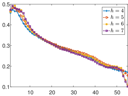
Figure 6: The MSE where \mathcal{D} is fully observed for PCA with different dimension sizes of the reduced space
