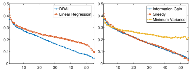
(a) Linear Regression and (b) Different heuristics of DRAL with IG
