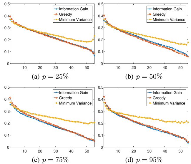
Figure 8: The MSE of different active selection methods for the DRAL model, where every entry of every record in \mathcal{D} is observed with probability p
